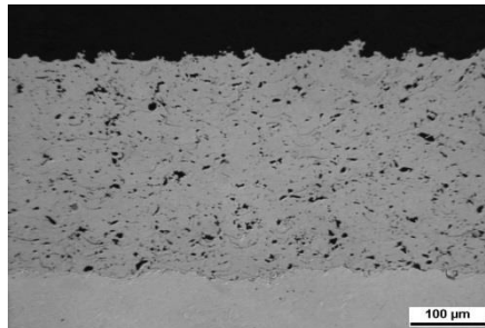
Typical microstructure of RocDur 44 sprayed with our Master Jet® flame spray gun.
